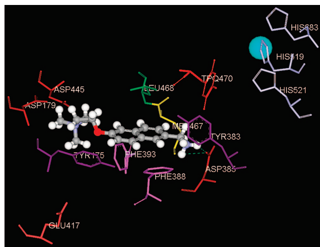
FIGURE 8. Best-scored productive docking mode of 12 with BPAO. Note that the substrate quaternary ammonium group is close to Asp445 to allow for an additional electrostatic interaction.
