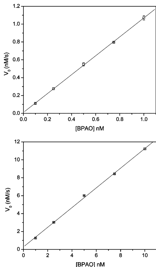
FIGURE 9. Linear relationship between enzyme concentration and initial oxidation velocity ( V_0 ) of 12 ( 10\ \mu\text{M} ) in 0.1\ \text{M} , \text{pH}\ 7.2 phosphate buffer at 30\ ^\circ\text{C} . Top: [\text{BPAO}] 0\text{--}1.00\ \text{nM} . Bottom: [\text{BPAO}] 1.00\text{--}10.0\ \text{nM} .
