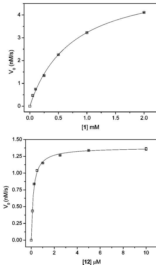
FIGURE 7. Plots of initial oxidation velocity ( V_0 ) versus substrate concentration of 1 in 33 mM, pH 7.2 phosphate buffer in the presence of BPAO (5.0 nM) (top) and of 12 in 0.1 M, pH 7.2 phosphate buffer in the presence of BPAO (2.0 nM) both at 30 ^{\circ}\text{C} (bottom) both at 30 ^{\circ}\text{C} as measured by fluorescence spectrophotometry.
