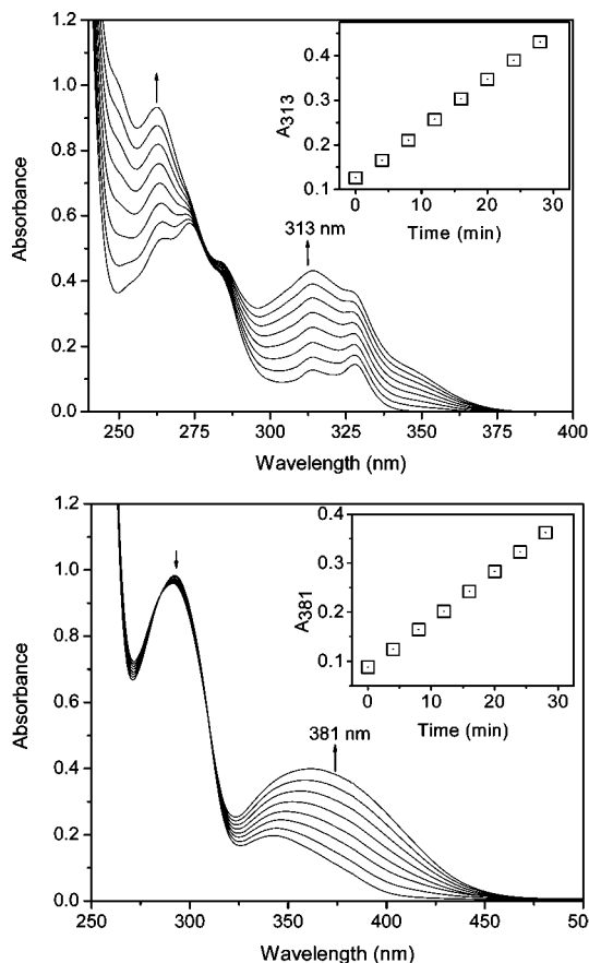
FIGURE 1. Time-dependent (4 min interval) UV-vis spectra recorded upon mixing 0.1 mM 1 (top) or 2 (bottom) with 0.1 \mu M BPAO in 0.1 M, pH 7.2 phosphate buffer at 30 °C. Insets: time-dependent plots of absorbance growth at wavelengths indicated.
