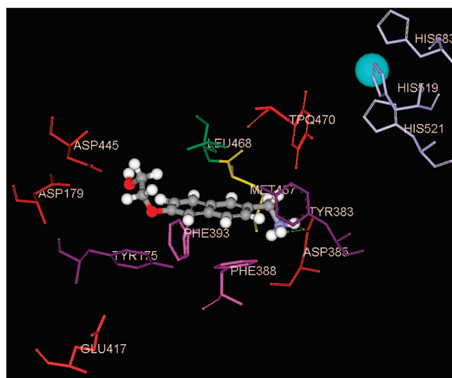
FIGURE 4. Best-scored productive docking mode of compound 7 with native BPAO. Note that the substrate OH is interacting with Asp445.
