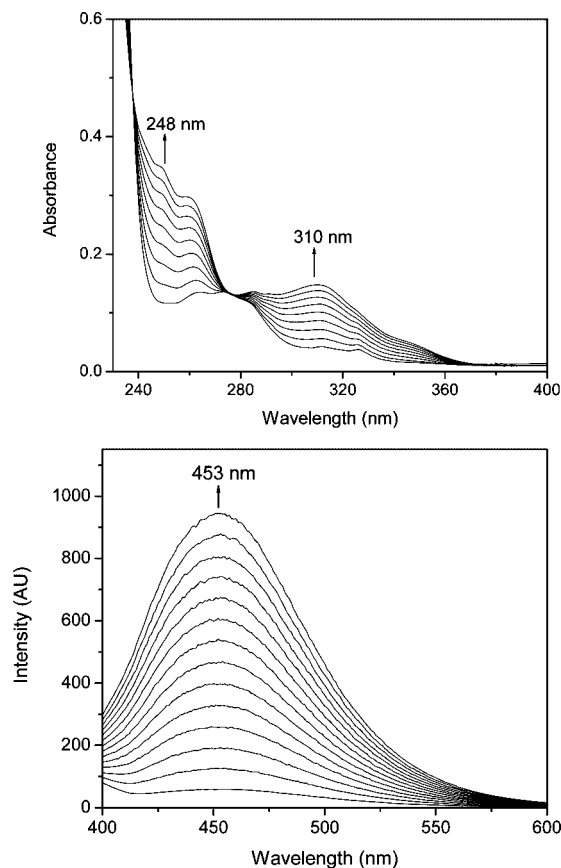
FIGURE 5. (Top) Time-dependent (30 s interval) UV-vis spectra recorded upon mixing 20 \mu M 12 with 0.1 \mu M BPAO in 0.1 M, pH 7.2 phosphate buffer at 30 °C. (Bottom) Time-dependent (1 min interval) fluorescence spectra ( \lambda_{\text{ex}} 350 nm) recorded upon mixing 12 (10 \mu M) with BPAO (1.0 nM) in 0.1 M, pH 7.2 phosphate buffer at 30 °C.
