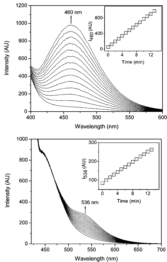
FIGURE 2. Time-dependent (1 min interval) fluorescence spectra recorded upon mixing 0.1 mM 1 (top) or 2 (bottom) with 5 nM BPAO in 0.1 M, pH 7.2 phosphate buffer at 30 °C. The \lambda_{\text{exc}} were 350 nm for 1 and 420 nm for 2 . Insets: time-dependent plots of emission growth at wavelengths indicated.
