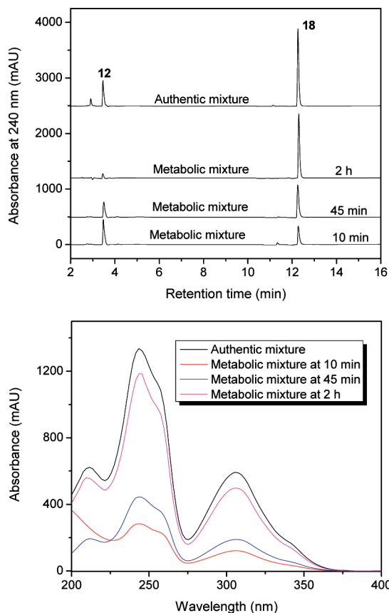
FIGURE 6. (Top) HPLC diagram of a mixture of authentic 12 and 18 (both 200 \mu\text{M} ), and time-dependent HPLC diagrams of a metabolic mixture of 12 (200 \mu\text{M} ) with BPAO (0.1 \mu\text{M} ) in 0.1 M, pH 7.2 phosphate buffer at 25 ^{\circ}\text{C} . (Bottom) Corresponding DAD spectra of peaks at 12.3 min ( 18 ).
